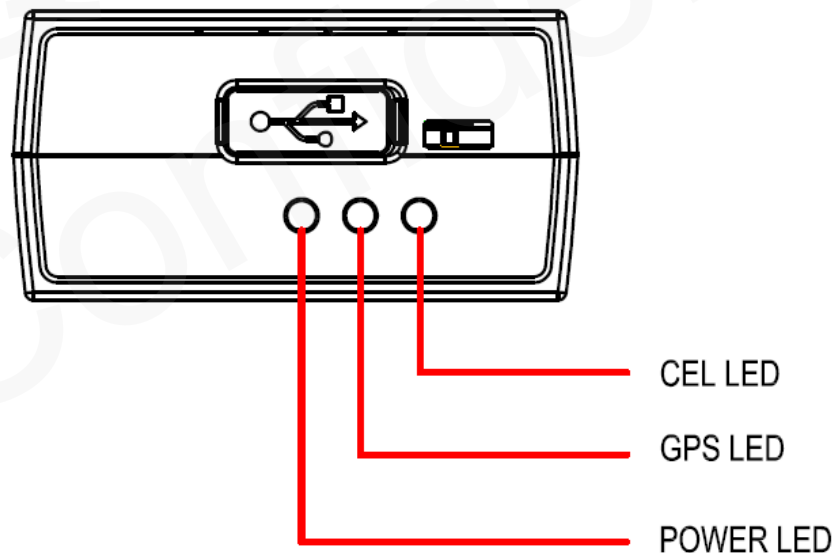
Figure 16. GV300W LED on the Case
